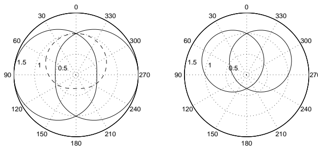
Figure 1: The cardioid panning method. In the left picture solid lines are right and left ear gains and a dashed line is front-back gain. In the right picture the final panning gains for left and right ear are depicted.
