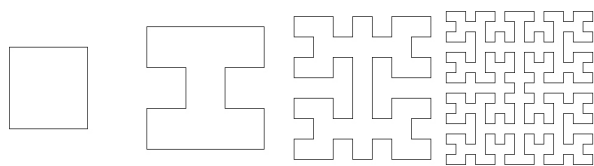
Figure 7: These are the first 4 iterations of the SFC introduced by Eliakim Moore. The Structure of this SFC is similar to Hilbert's SFC but more symmetric which leads to interesting properties for interactive sonification.
