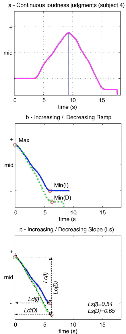
Figure 2. a) Continuous loudness profile obtained by subject 4 for a ramp duration of 5 s. b) Superposition of increasing and decreasing profiles. c) Slopes obtained by linear regression of the continuous rating profiles.
