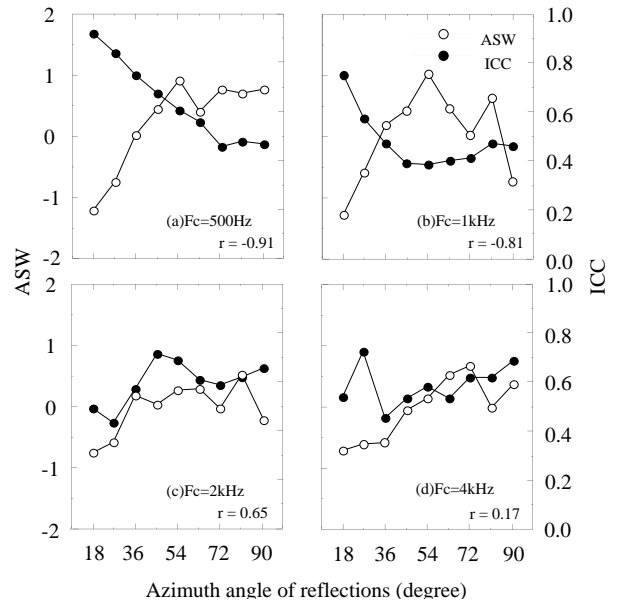
Figure 11. ASW and measured ICC for 1/1 oct. band noise as a function of azimuth angle of lateral reflections. The parameter is the center frequency.
