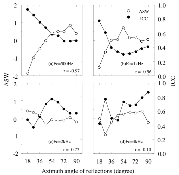
Figure 12. ASW and measured ICC for 1/3 oct. band noise as a function of azimuth angle of lateral reflections. The parameter is the center frequency.
